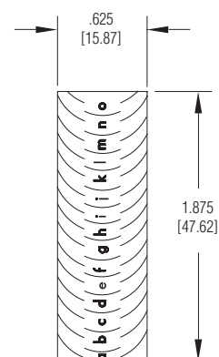
Trimable Vane
