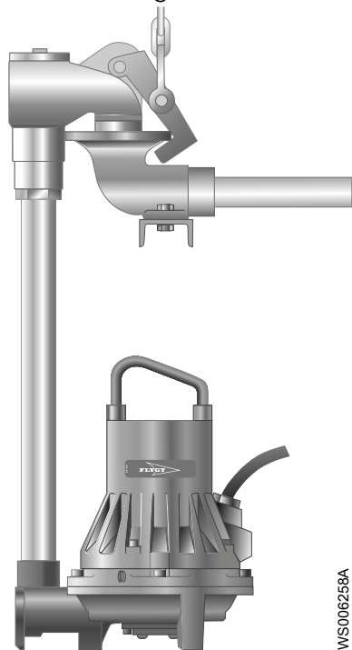
Figur 8: H-installation
