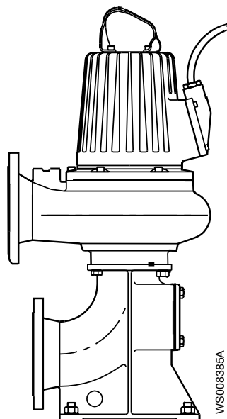
Figur 4: T-installation
