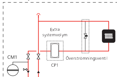
Radiatorsystem
