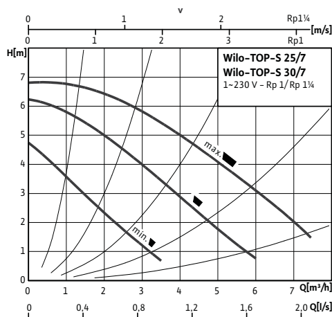
Pumpkurva TOP-S 25/7 (CTC EcoHeat 306-310)
