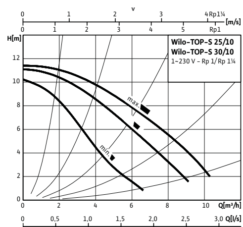
Pumpkurva TOP-S 25/10 (CTC EcoHeat 312)
