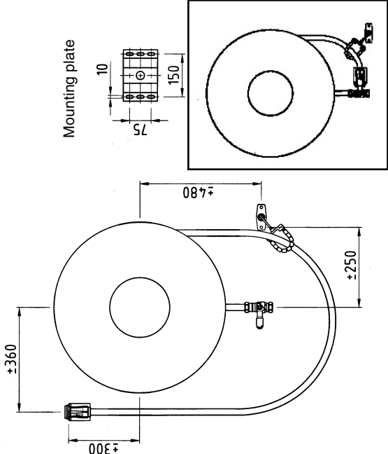
Fixed rigid installation kit on wall.
