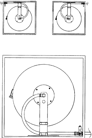
Swinging installation kit fitted in cabinet
