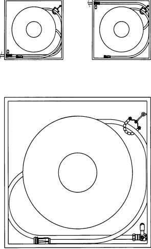
Flexible installation kit, 3 different positions of the feeding valve in the cabinet are possible.
