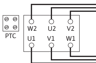
Fig. 16: Y-Δ-koppling
