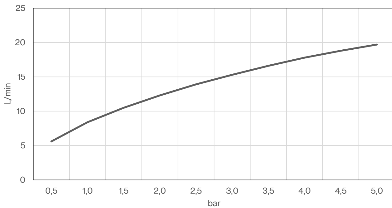
QST1150 flow rate (without aerator)
