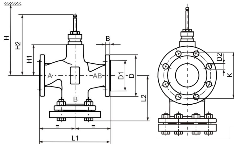
Valve, DN150
