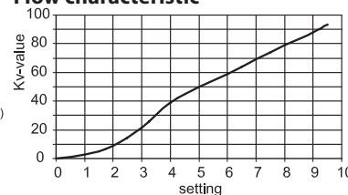
Flow characteristic
