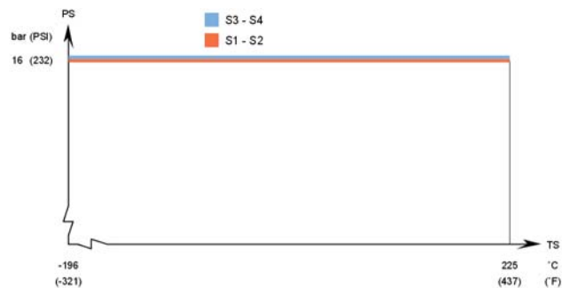
CB20 – PED approval pressure/temperature graph
