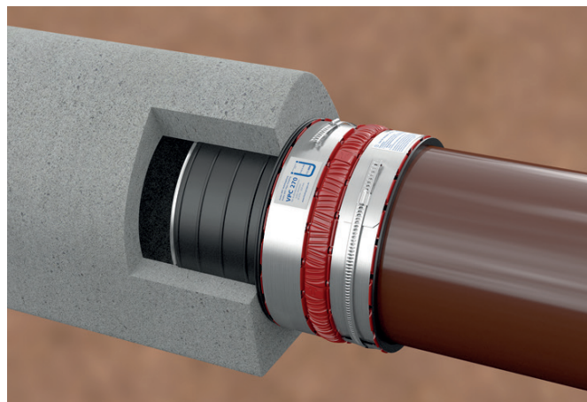
BI-Adapter, montageexempel
