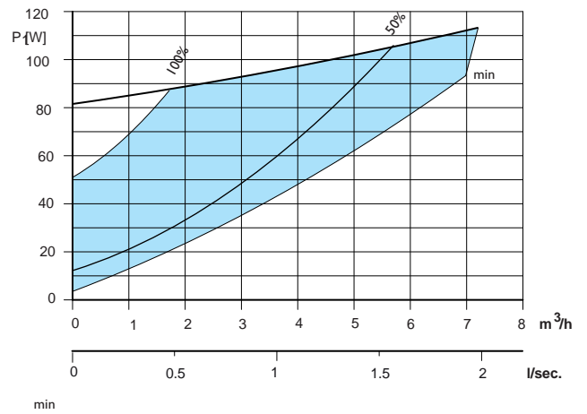
Calio 30-60, Boost
