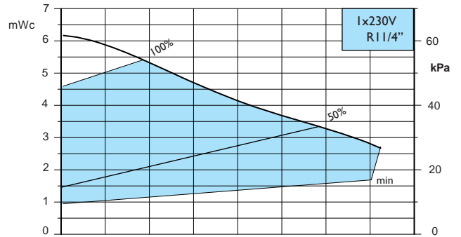
Calio 30-60, Δ pv
