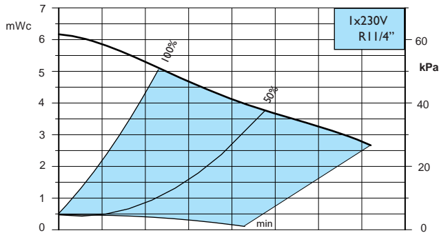
Calio 30-60, ECO
