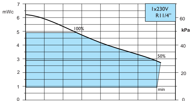
Calio 30-60, Δpc
