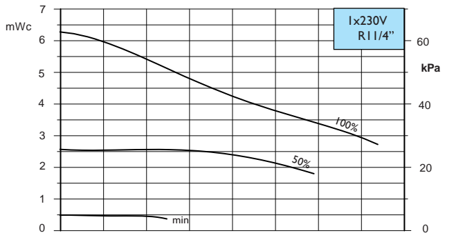
Calio 30-60, Boost
