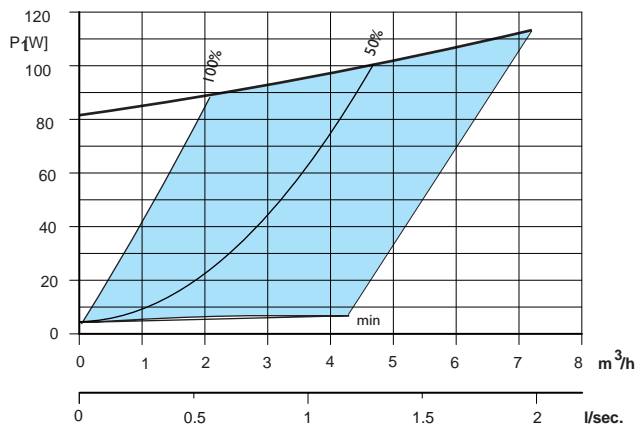
Calio 30-60, Δpc
