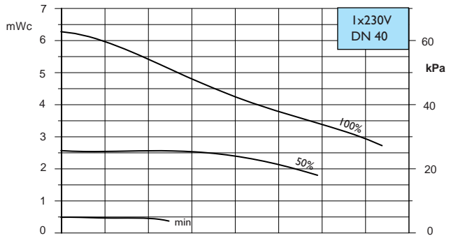
Calio 40-60, Boost
