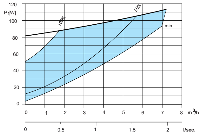
Calio 40-60, Boost
