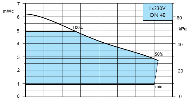
Calio 40-60, Δpc
