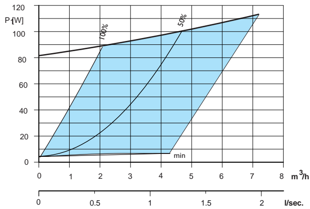
Calio 40-60, Δpc
