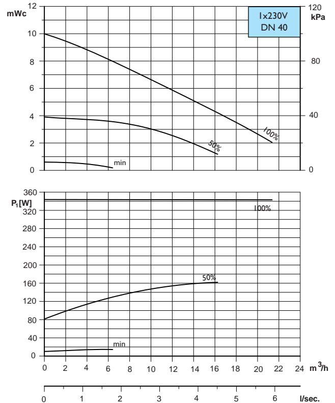
Calio 40-100, Boost
