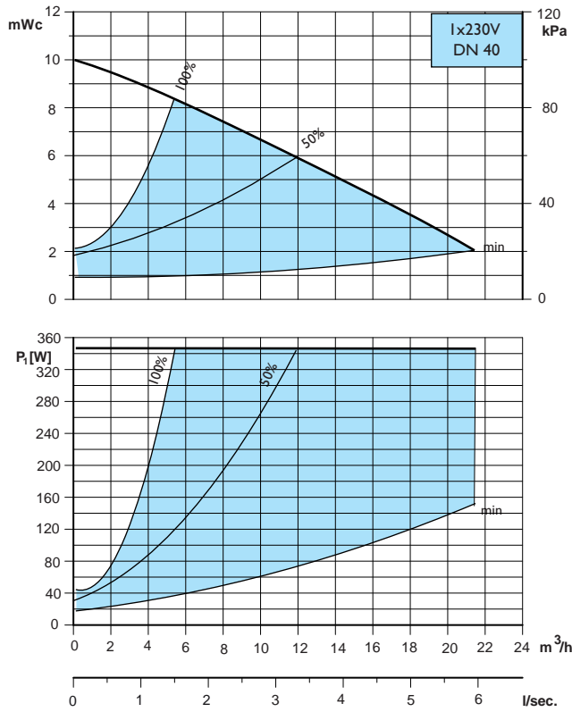
Calio 40-100, ECO
