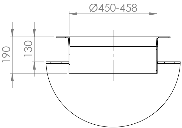
DETAIL C
