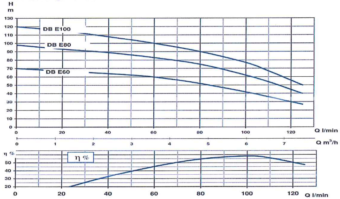
PERFORMANCE CHARACTERISTICS AT 2850 rpm
