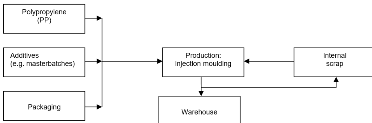
Figure 2. Diagram of the manufacturing process of production site Kartoszyno.
