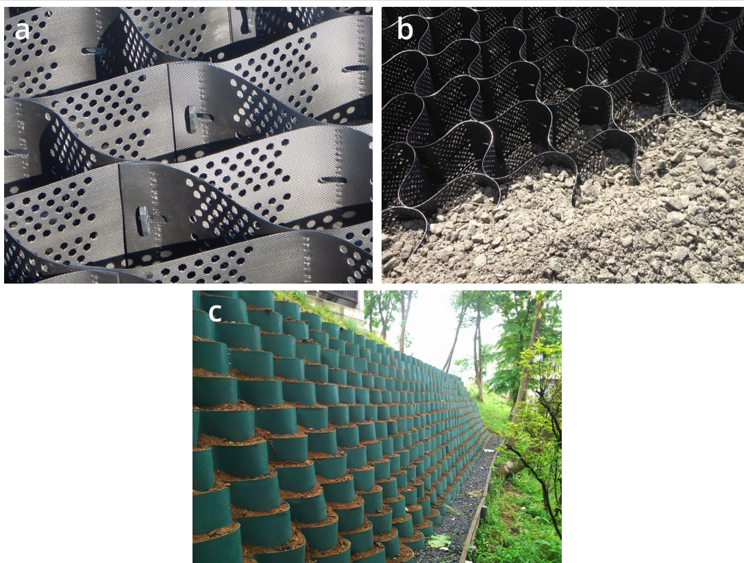
Figure 1. Product Images of GEOWEB® Geocell (a) Genuine, (b) Alpha, and (c) Wall products
