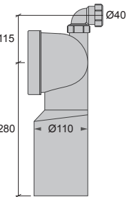
C + K3 WC - Stos, Universal, X-tra RSK 310 66 83
