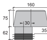
A GAS - WC 30, Excentrisk 30 mm RSK 310 67 10 NRF 619 66 69 LVI 56 884 41
