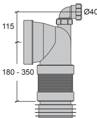
A WC - Stos, Universal X-tra, Flexibel RSK 310 67 27
