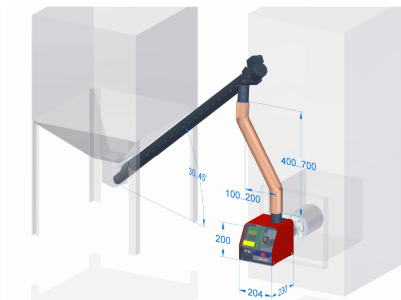
Figur 11 Externskruvens placering
