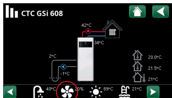
Menu "Operation".
