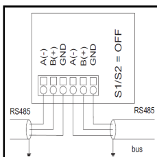
Figure 7.2.1 wiring in line RS485
