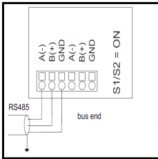
Figure 7.2.2 wiring end of line RS485
