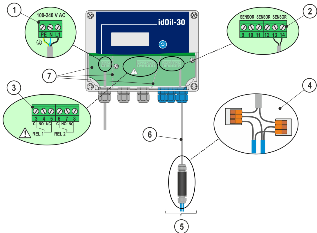
Figure 13. Connection with a two-sensor cable connector
