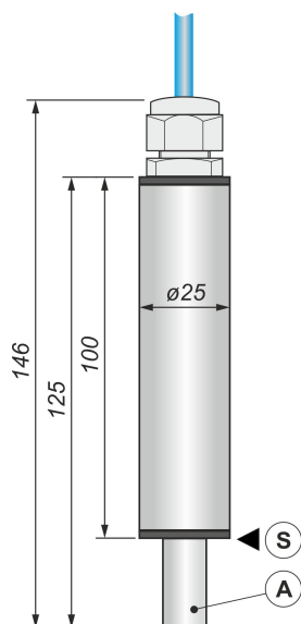
Figure 3. High liquid level sensor idOil-LIQ – structure and dimensions (mm)
