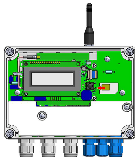
Figure 21. SIM card installation
