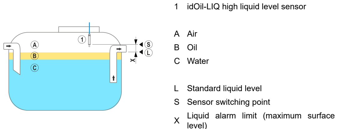
Figure 9. Installing the idOil-LIQ high liquid limit sensor
