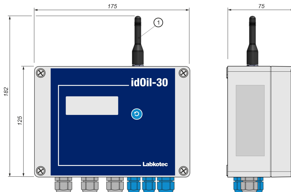
1 idOil-30 3G model with antenna (option)
