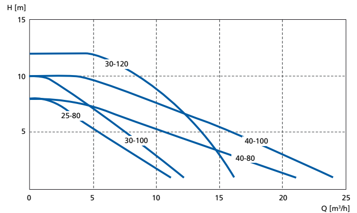
Calio-Therm pumpkurva
