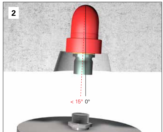
2) This requires a special adjusting tool. It is important to ensure that the bending radius is not more than 15°. The bearing surface of the female thread serves as a reference point on the surface.
