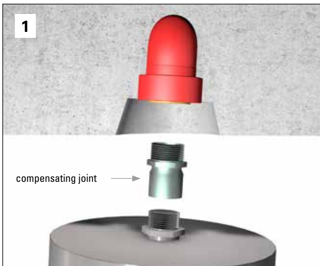
1) If the sprinkler connection protrudes obliquely from the concrete surface, it is possible to align this with the balancing connection. The balancing connection is installed with the provided hexagon in the sprinkler connection thread. A common sealing method for the preparation of waterproof threaded connections is to be used.
