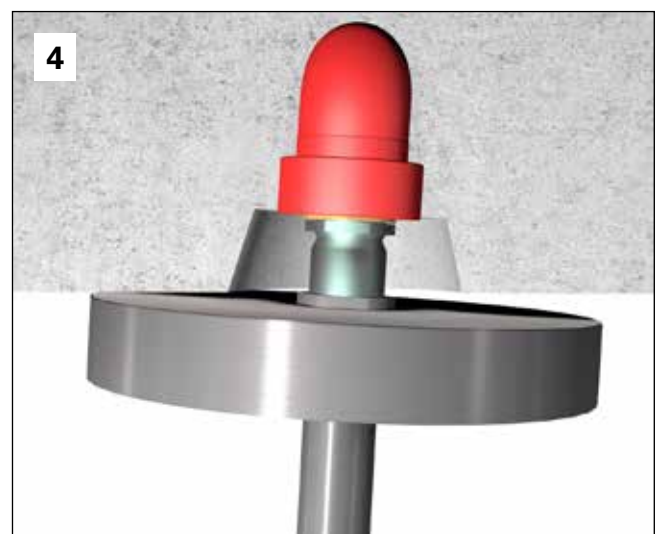
4) With gentle pressure by hand, the compensating joint is pushed into its position until the plate of the adjusting tool fits proper against the concrete surface.
