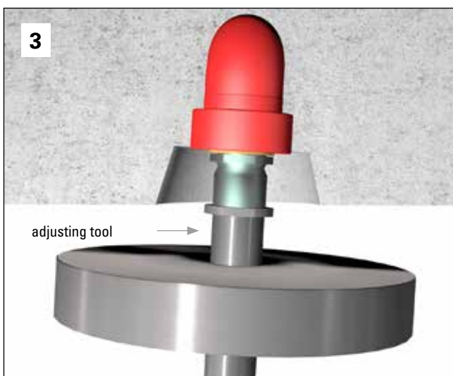
3) The adjusting tool is screwed into the balancing connection with the appropriate adapter.
