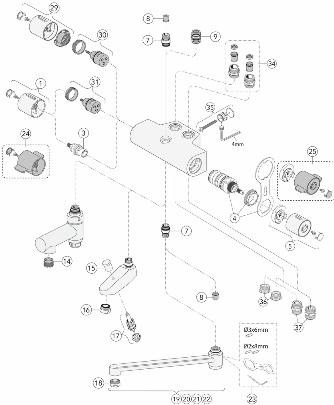
ExplodedView New Nautic_thermomixer_40cc_mixers (Rev 1. 2023-02-07)
