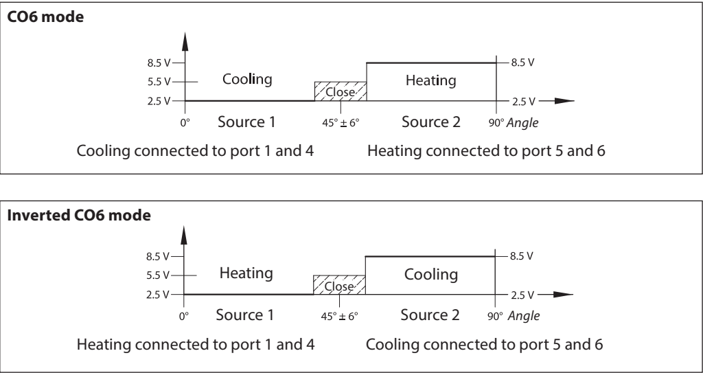
Signal from NovoCon® S to the Actuator NovoCon® ChangeOver 6
