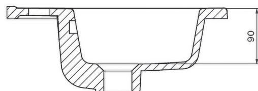
A-A (1/3)
