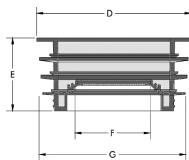
Universalkoppling
