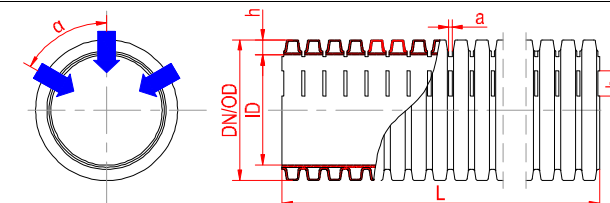
Multipurpose pipe MP(≤120°)
