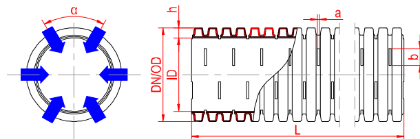
Locally perforated pipe LP(180°±10°)
