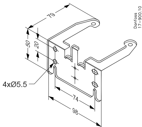
1. Mounting bracket, code number 017B1018, for direct mounting on the wall
