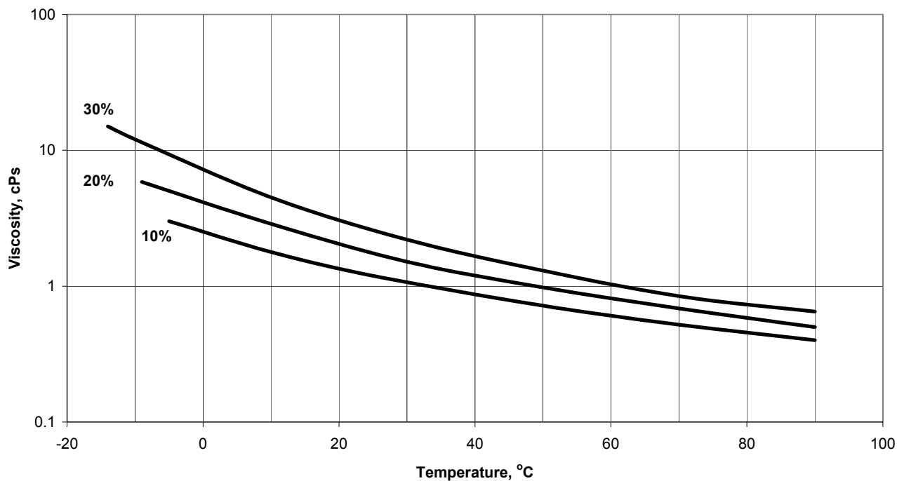
Viscosity Chart
