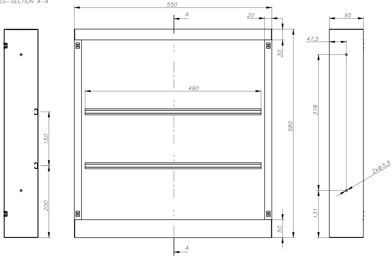
CROSS-SECTION A-A
