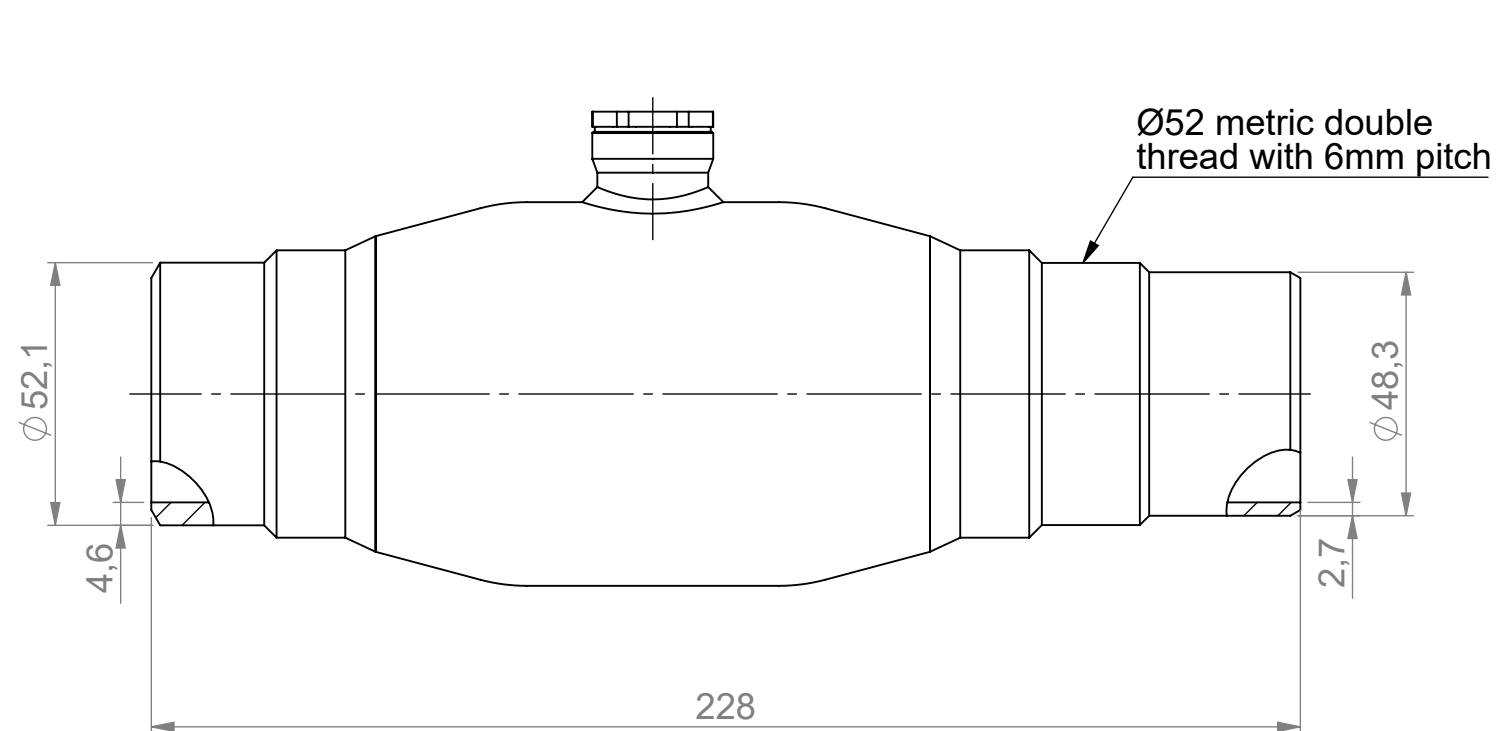
Top view of the stem without the plug
